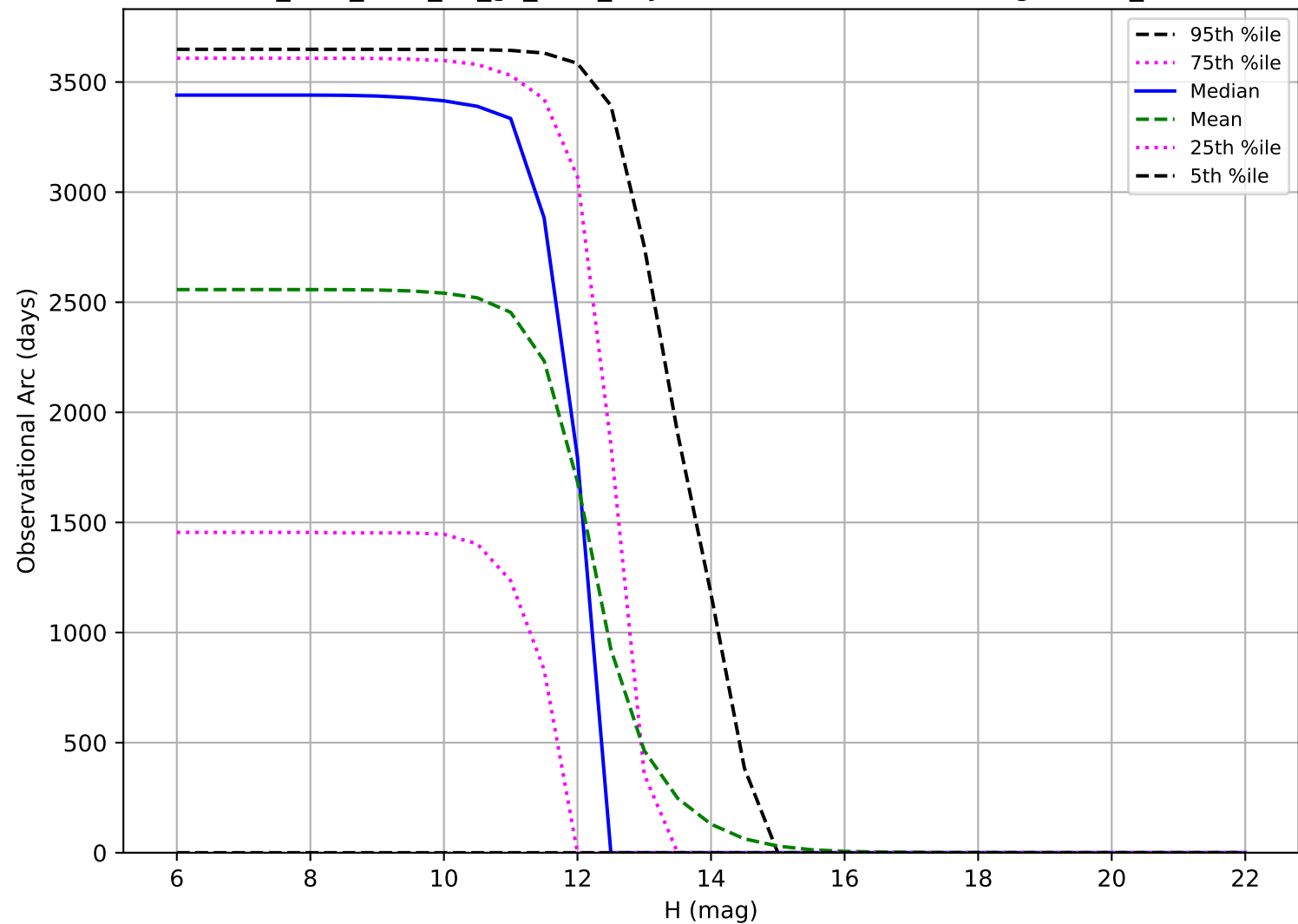
too_elab_r128_d3_gz_v3.4_10yrs: Observational Arc Length OCC_r20
