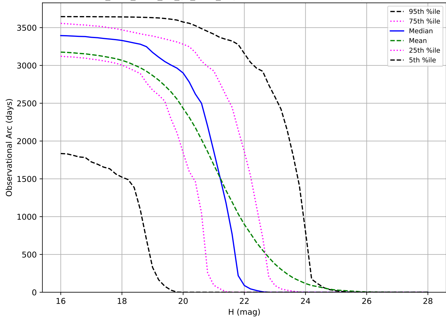
too_elab_r128_d3_gz_v3.4_10yrs: Observational Arc Length NEO
