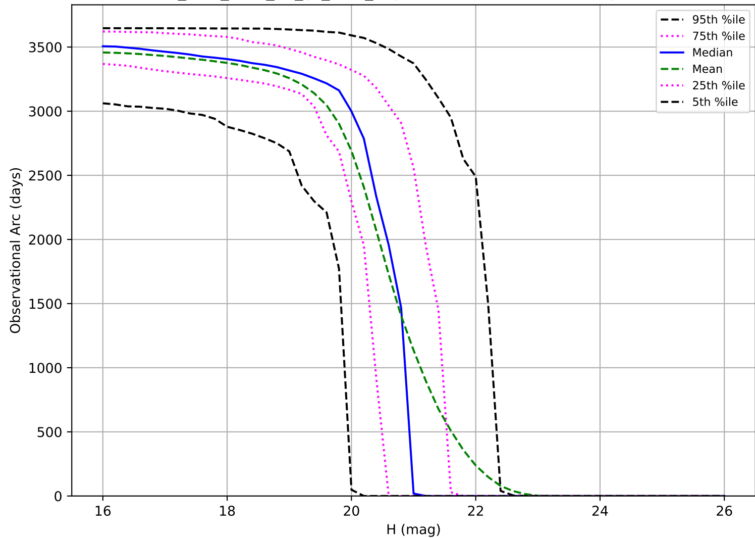
too_elab_r128_d3_gz_v3.4_10yrs: Observational Arc Length MBA
