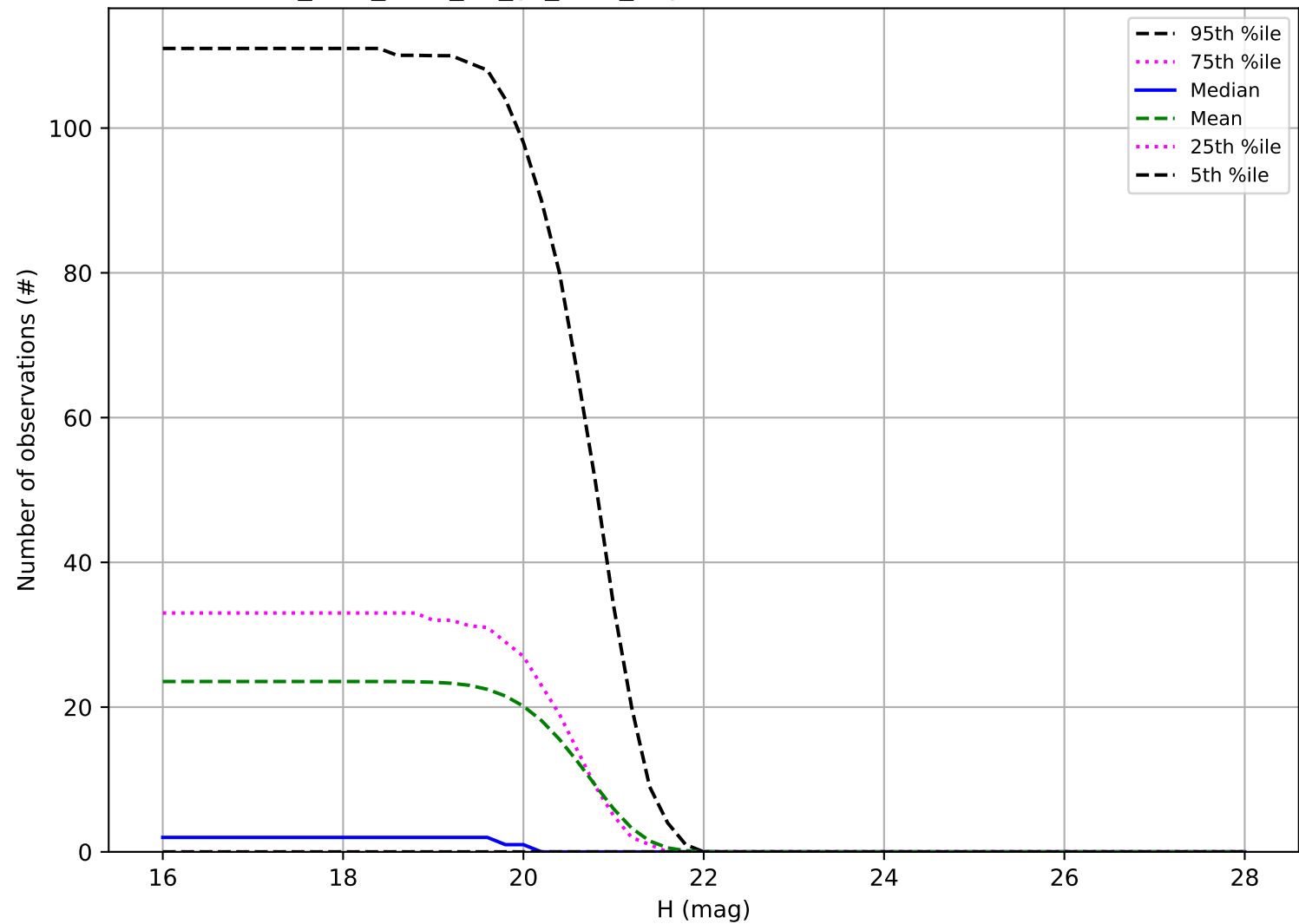
too_elab_r128_d3_gz_v3.4_10yrs: Number of observations Vatira
