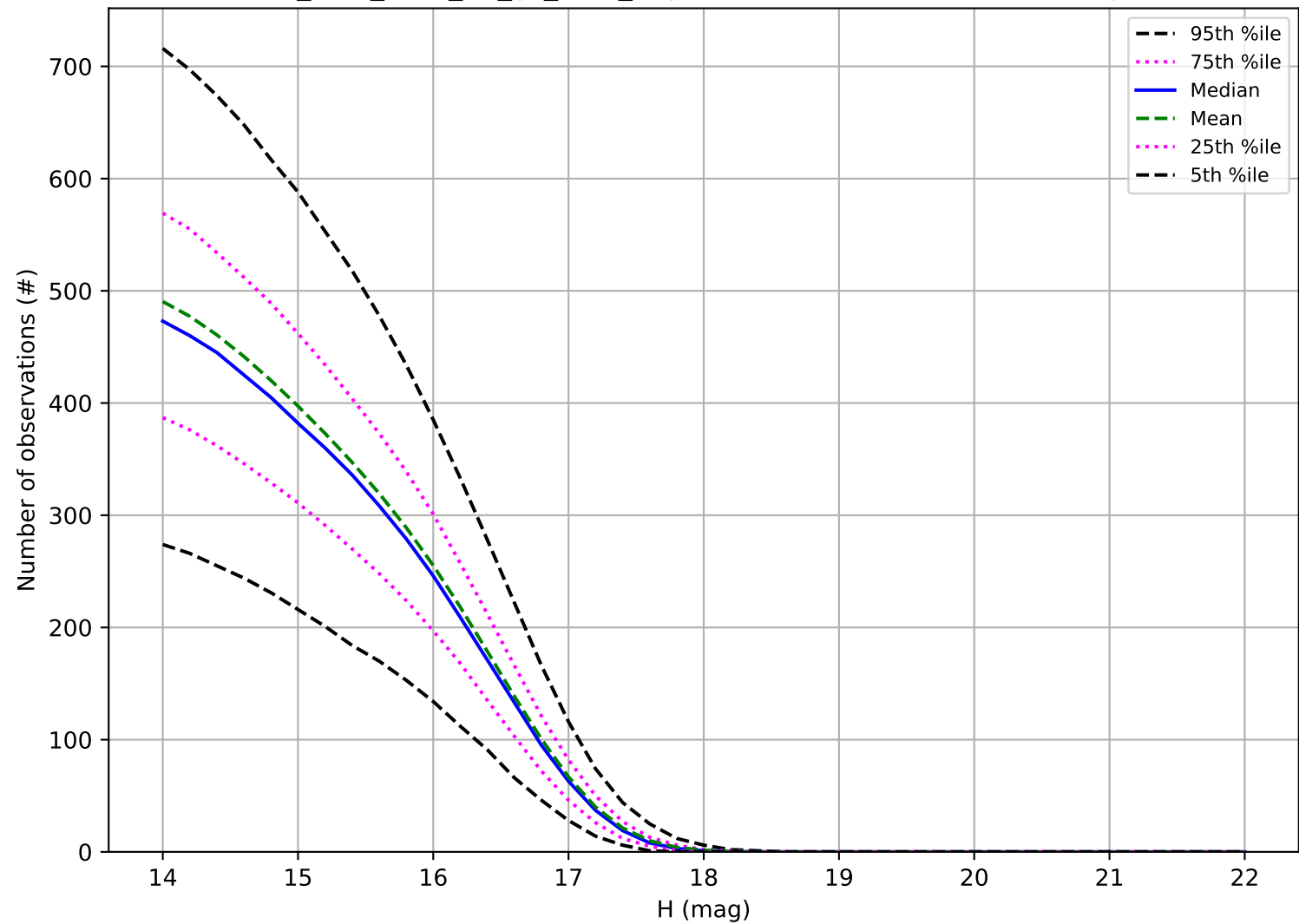
too_elab_r128_d3_gz_v3.4_10yrs: Number of observations Trojan
