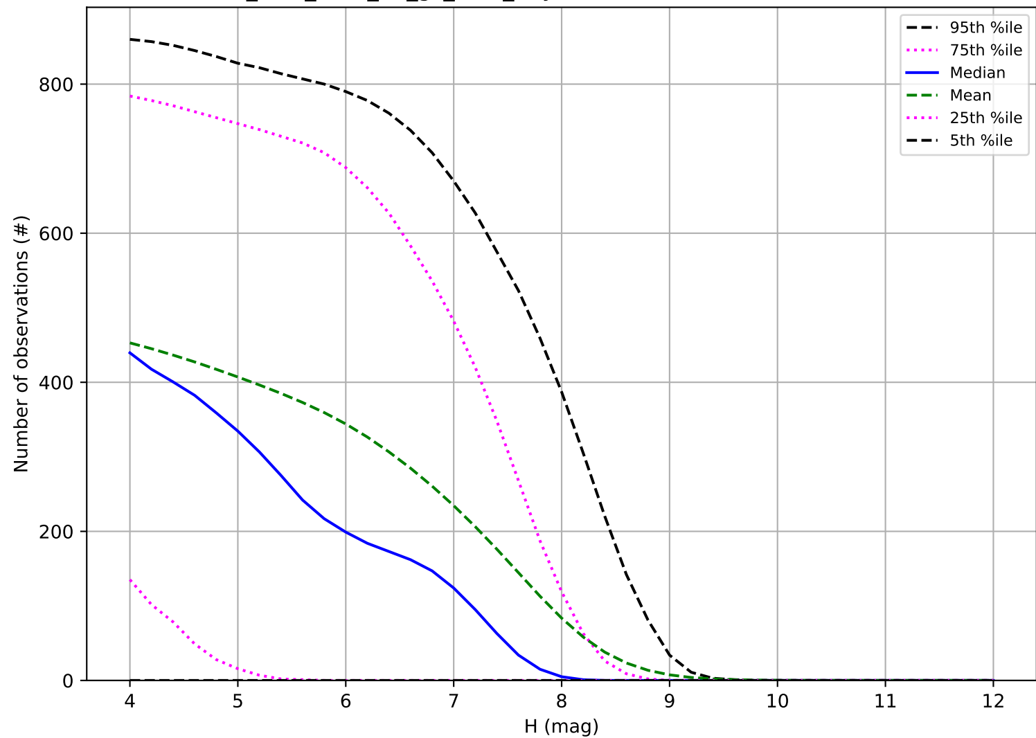
too_elab_r128_d3_gz_v3.4_10yrs: Number of observations TNO
