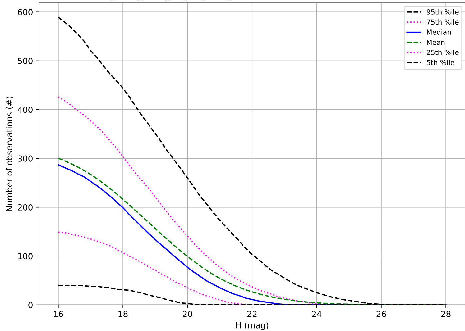
too_elab_r128_d3_gz_v3.4_10yrs: Number of observations PHA
