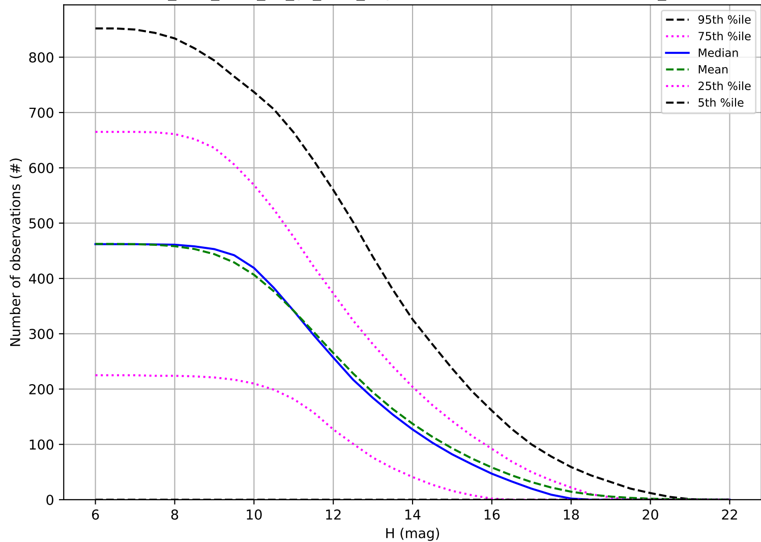
too_elab_r128_d3_gz_v3.4_10yrs: Number of observations OCC_r5
