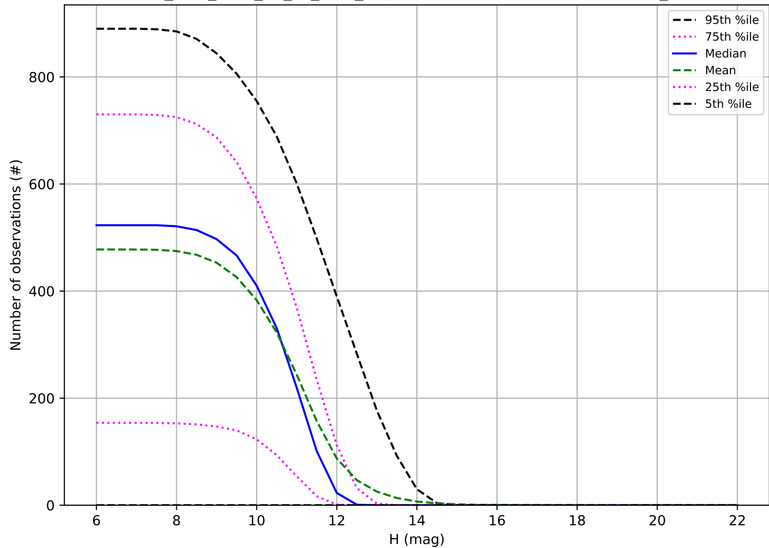
too_elab_r128_d3_gz_v3.4_10yrs: Number of observations OCC_r20
