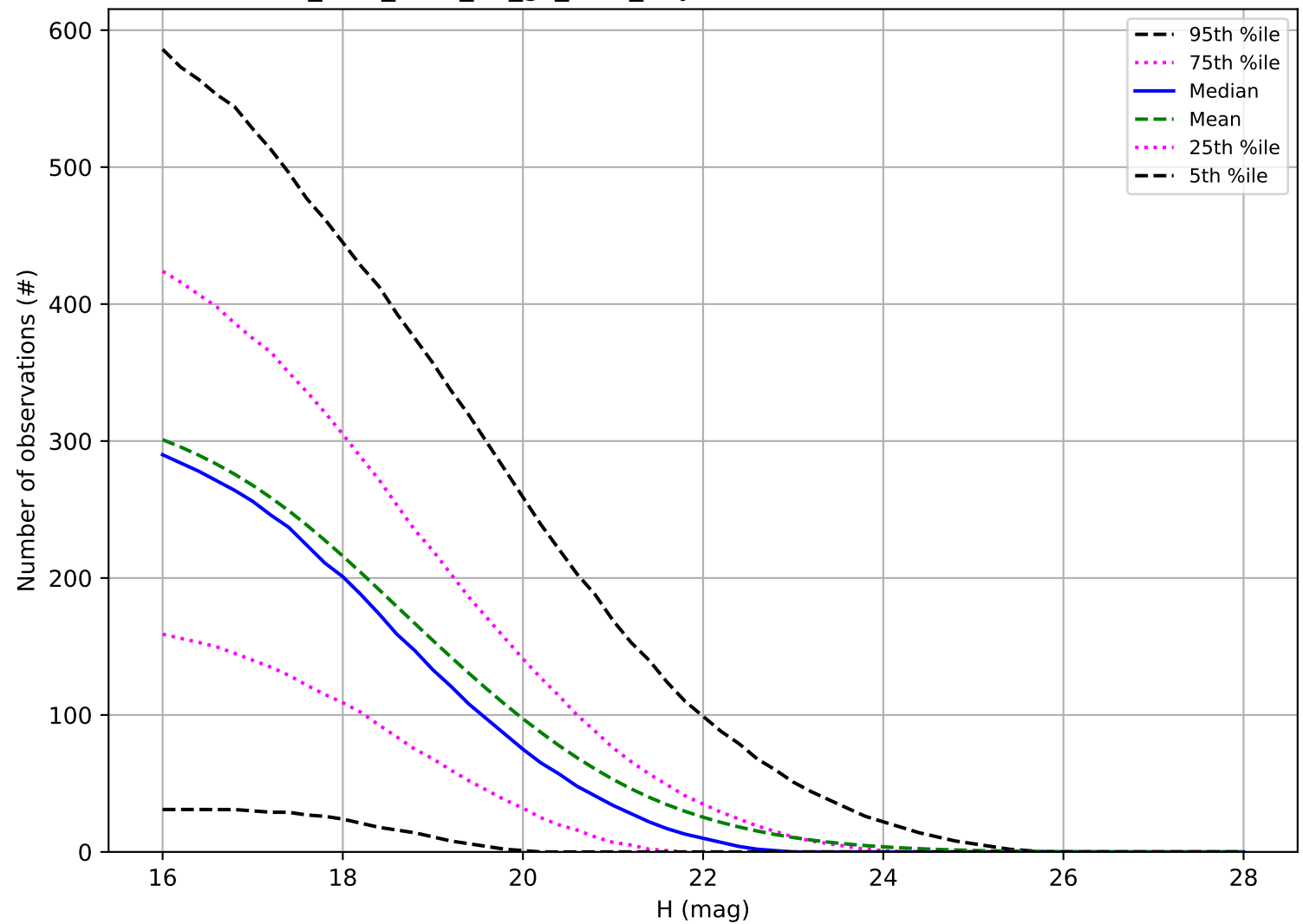
too_elab_r128_d3_gz_v3.4_10yrs: Number of observations NEO
