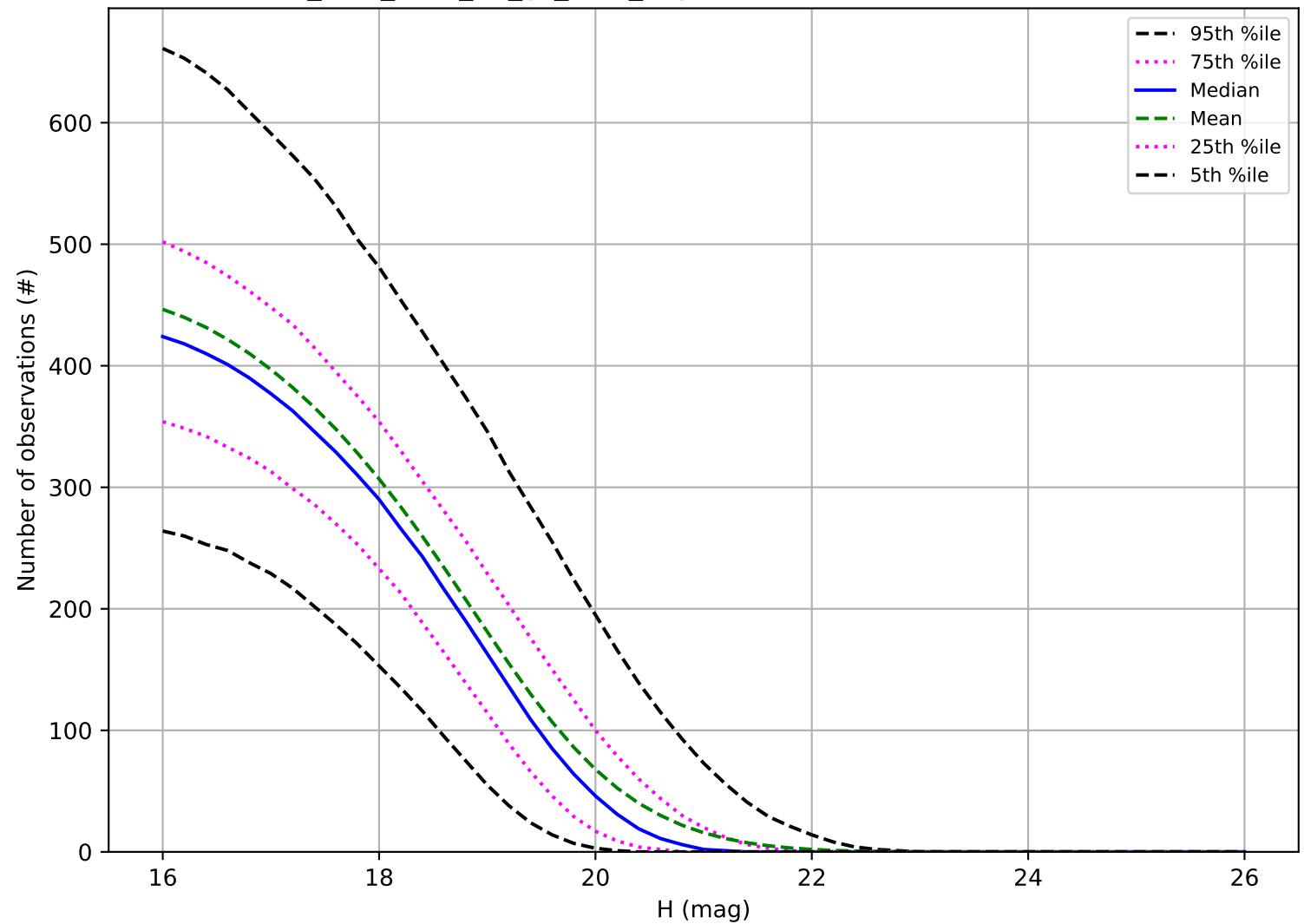
too_elab_r128_d3_gz_v3.4_10yrs: Number of observations MBA
