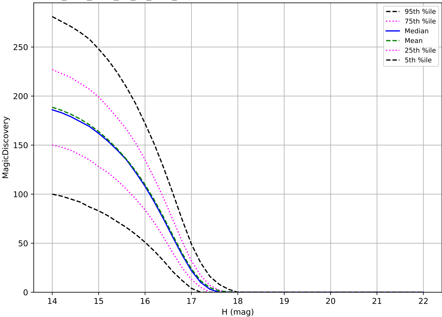
too_elab_r128_d3_gz_v3.4_10yrs: Trojan 6 detections in 60 nights detection loss
