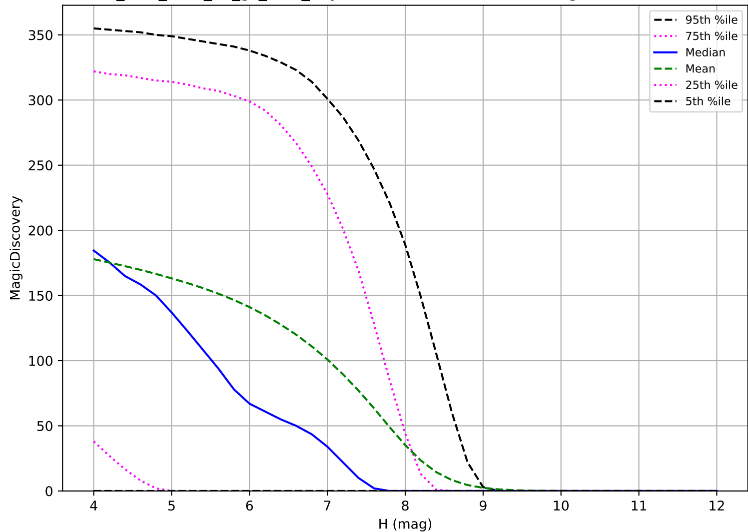
too_elab_r128_d3_gz_v3.4_10yrs: TNO 6 detections in 60 nights detection loss
