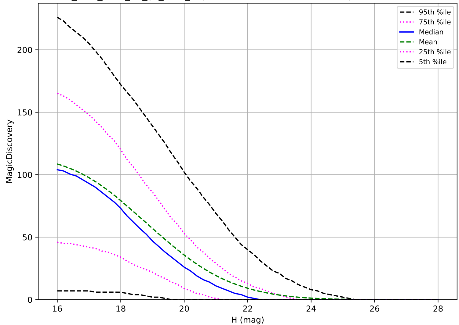
too_elab_r128_d3_gz_v3.4_10yrs: PHA 6 detections in 60 nights detection loss
