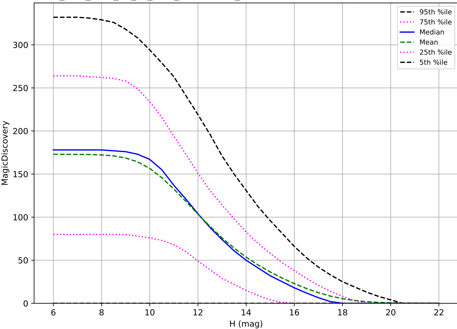
too_elab_r128_d3_gz_v3.4_10yrs: OCC_r5 6 detections in 60 nights detection loss
