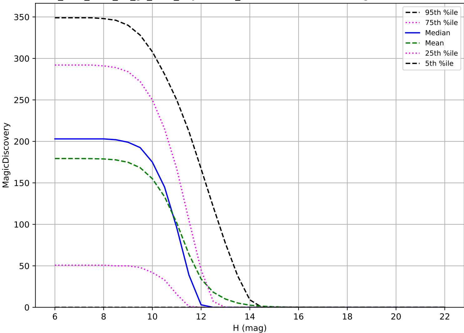
too_elab_r128_d3_gz_v3.4_10yrs: OCC_r20 6 detections in 60 nights detection loss
