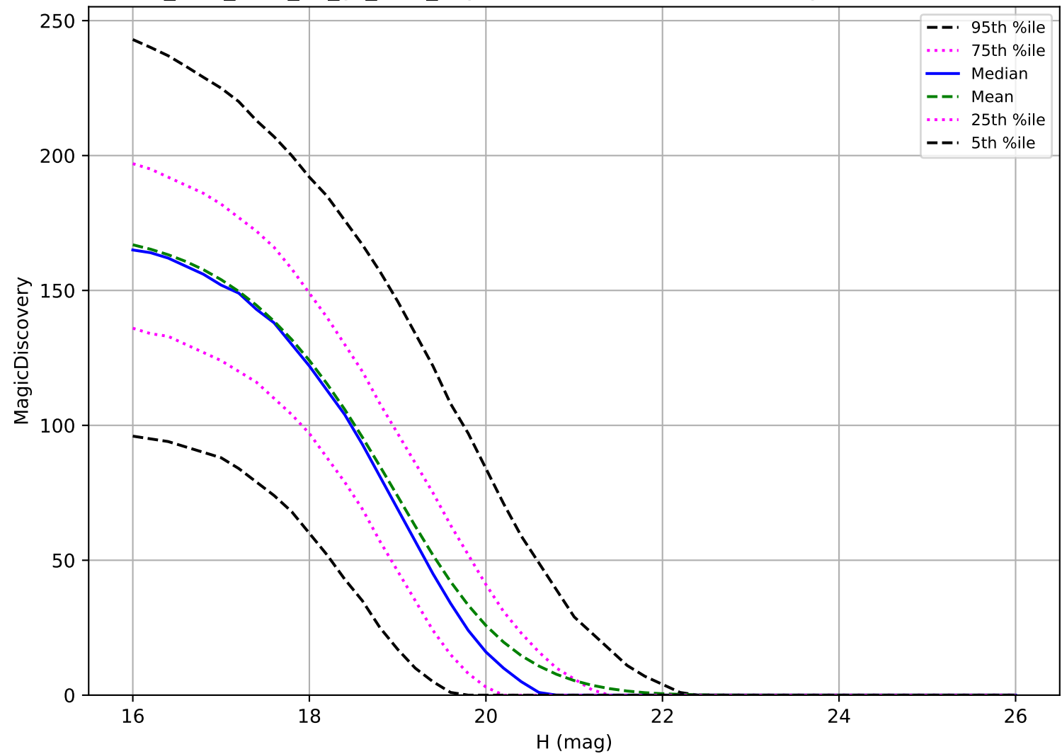
too_elab_r128_d3_gz_v3.4_10yrs: MBA 6 detections in 60 nights detection loss
