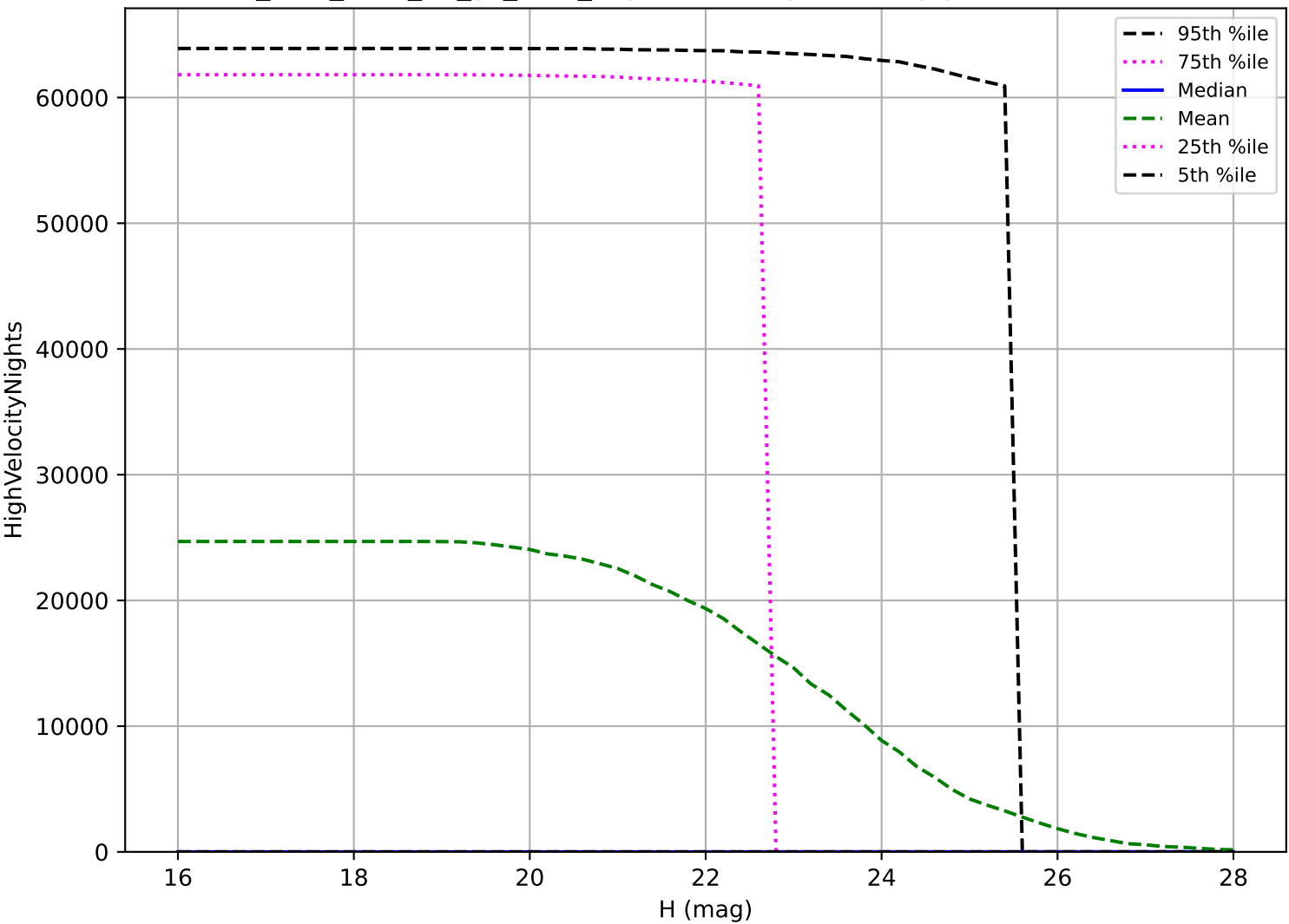
too_elab_r128_d3_gz_v3.4_10yrs: PHA High velocity pair detection loss
