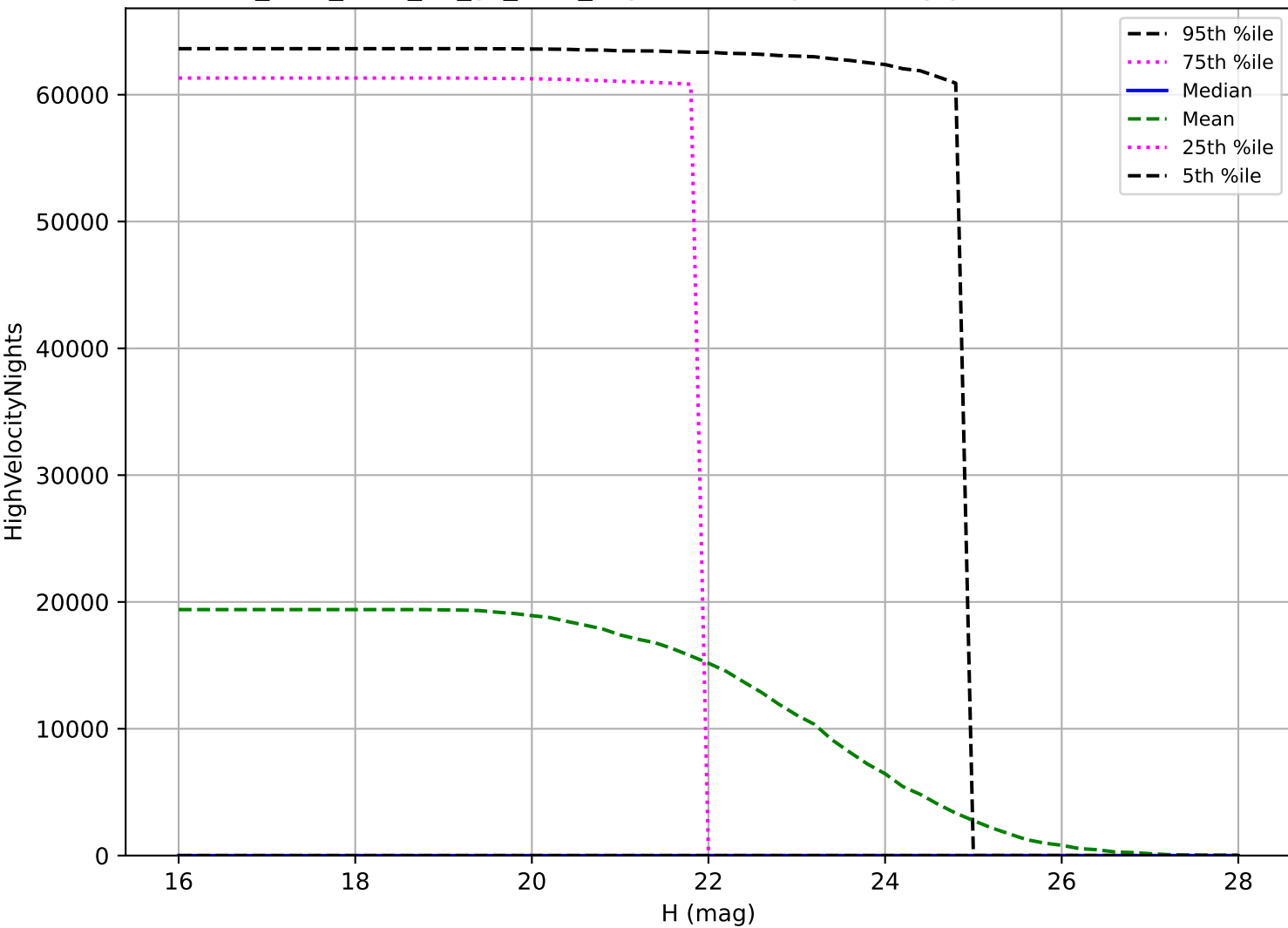
too_elab_r128_d3_gz_v3.4_10yrs: NEO High velocity pair detection loss
