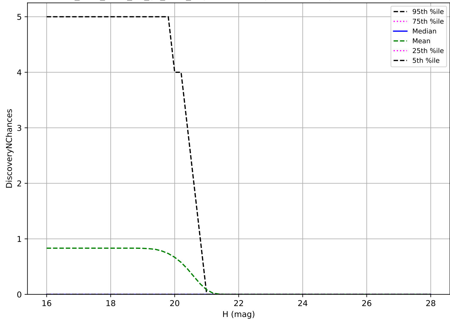
too_elab_r128_d3_gz_v3.4_10yrs: Vatira 3 pairs in 15 nights detection loss
