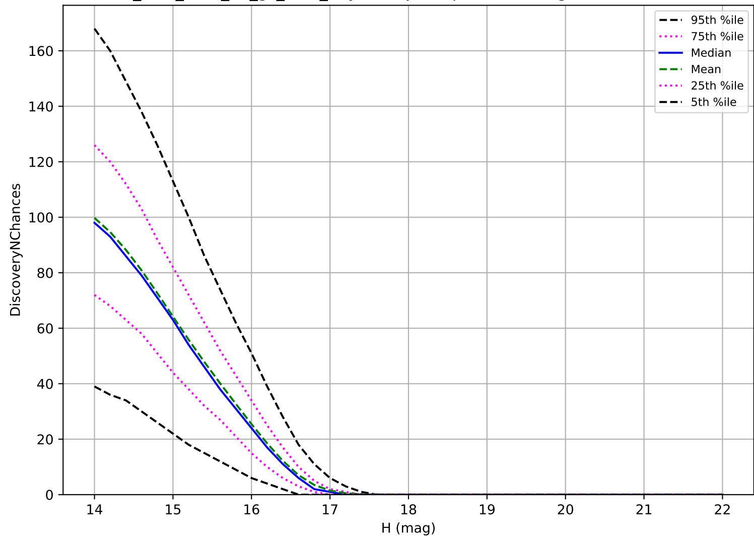
too_elab_r128_d3_gz_v3.4_10yrs: Trojan 3 pairs in 15 nights detection loss
