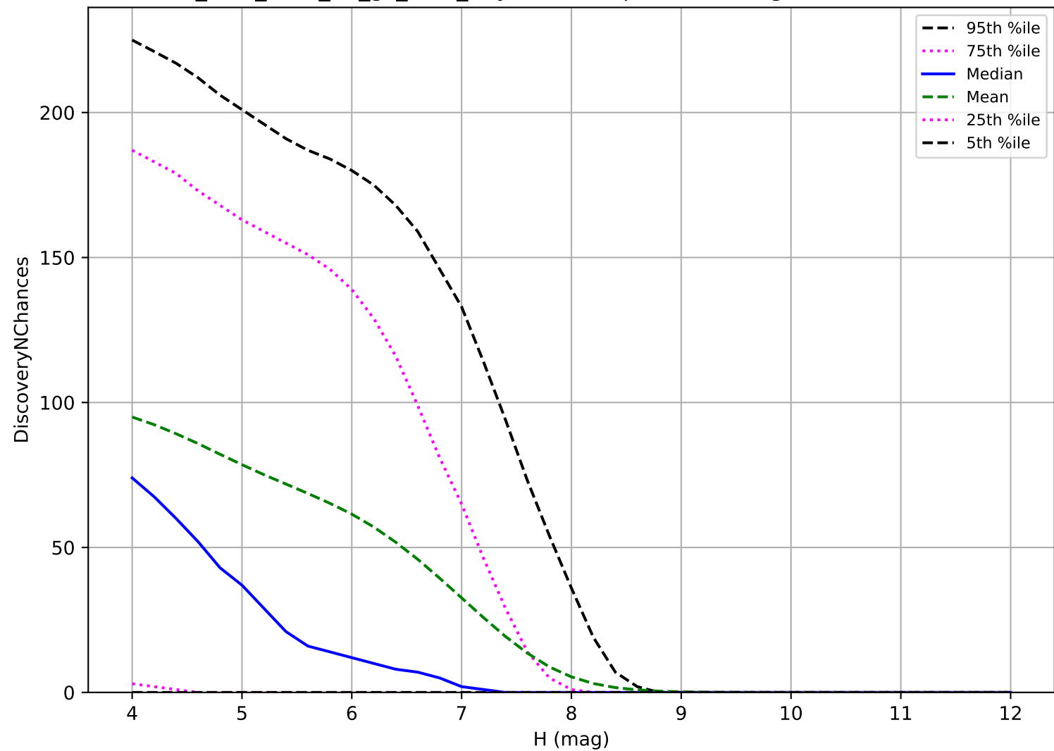
too_elab_r128_d3_gz_v3.4_10yrs: TNO 3 pairs in 15 nights detection loss
