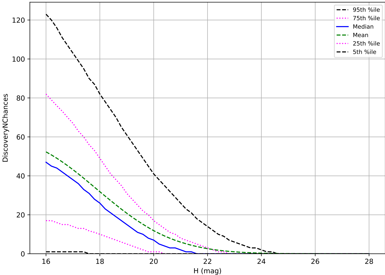
too_elab_r128_d3_gz_v3.4_10yrs: PHA 3 pairs in 15 nights detection loss
