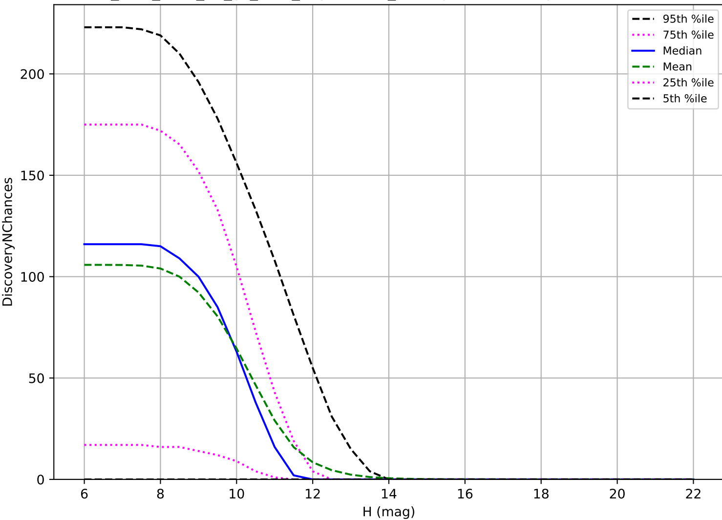
too_elab_r128_d3_gz_v3.4_10yrs: OCC_r20 3 pairs in 15 nights detection loss
