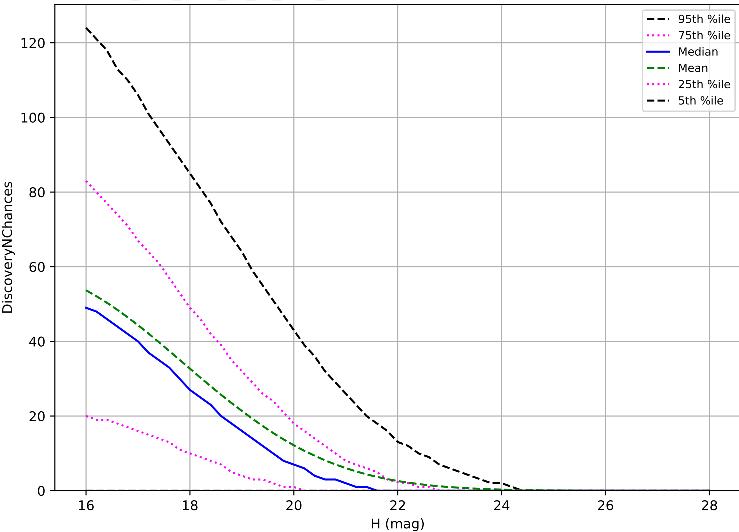
too_elab_r128_d3_gz_v3.4_10yrs: NEO 3 pairs in 15 nights detection loss
