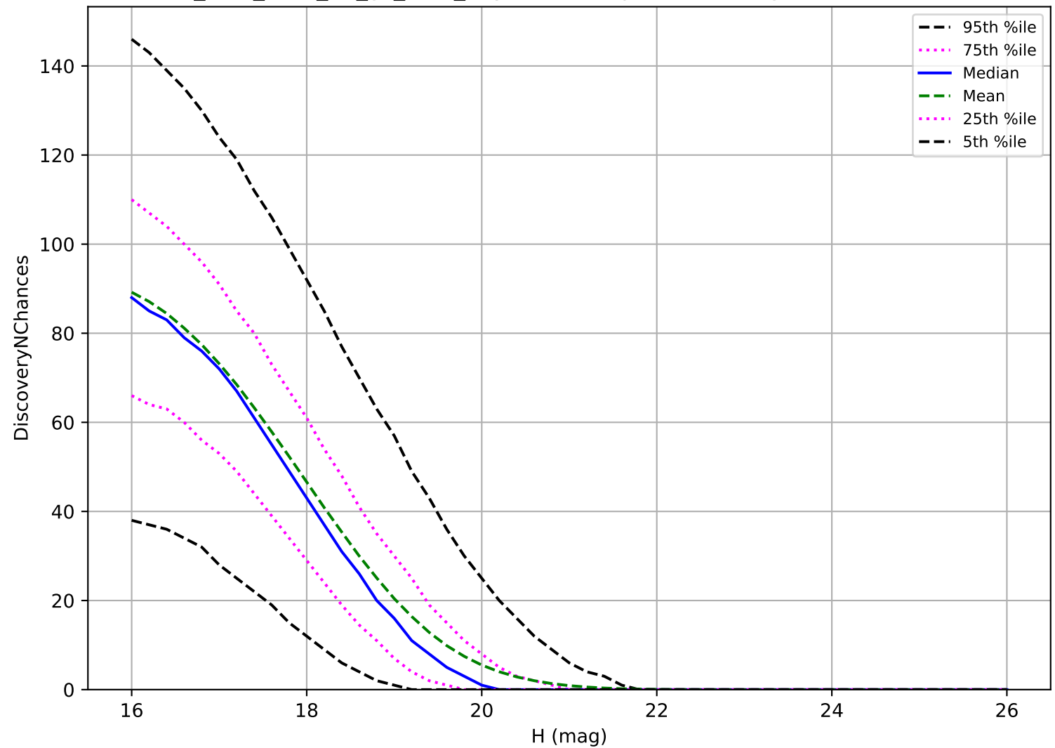
too_elab_r128_d3_gz_v3.4_10yrs: MBA 3 pairs in 15 nights detection loss
