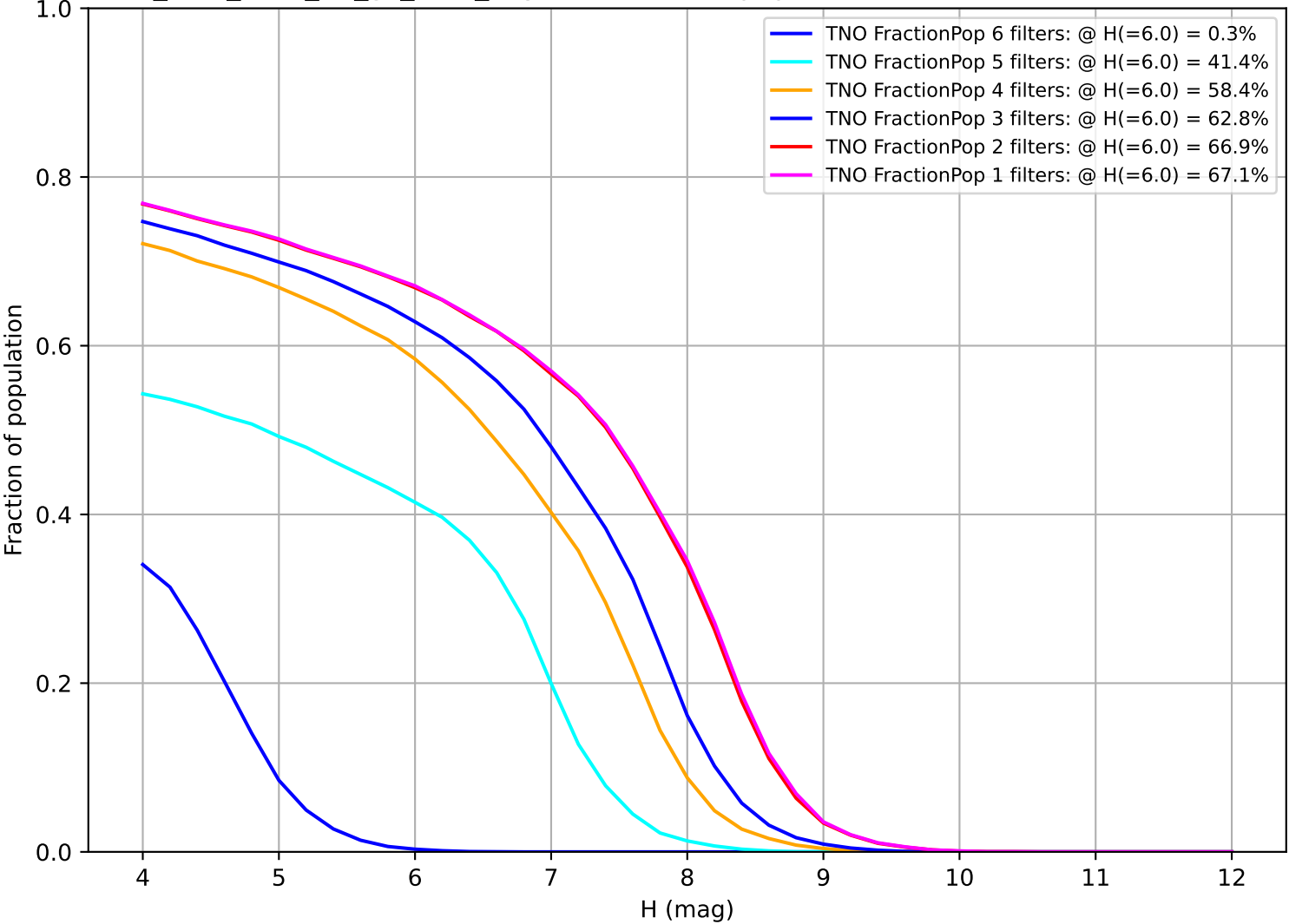
too_elab_r128_d3_gz_v3.4_10yrs: Fraction of population with colors in X filters TNO
