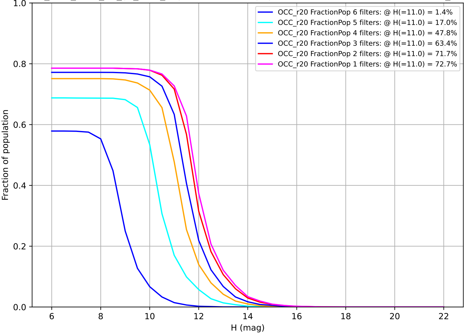
too_elab_r128_d3_gz_v3.4_10yrs: Fraction of population with colors in X filters OCC_r20
