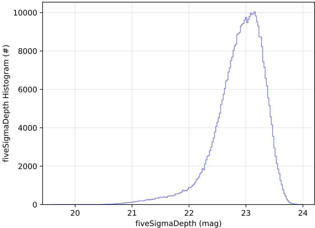
too_elab_r128_d3_gz_v3.4_10yrs z: fiveSigmaDepth Histogram
