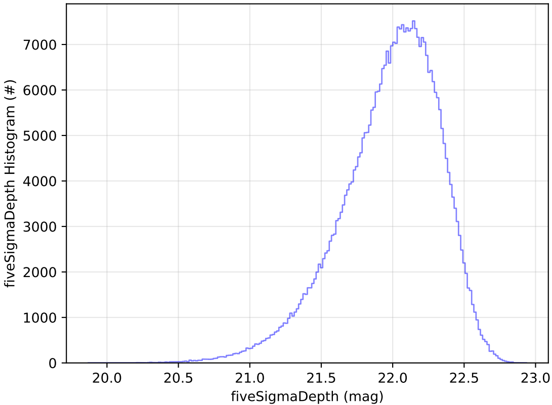
too_elab_r128_d3_gz_v3.4_10yrs y: fiveSigmaDepth Histogram
