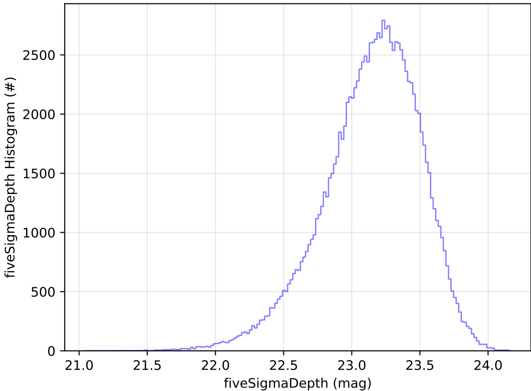
too_elab_r128_d3_gz_v3.4_10yrs u: fiveSigmaDepth Histogram
