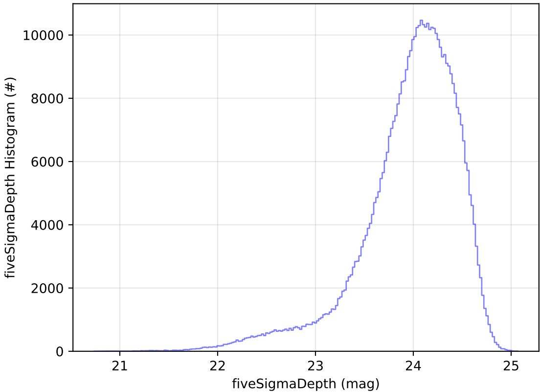
too_elab_r128_d3_gz_v3.4_10yrs r: fiveSigmaDepth Histogram
