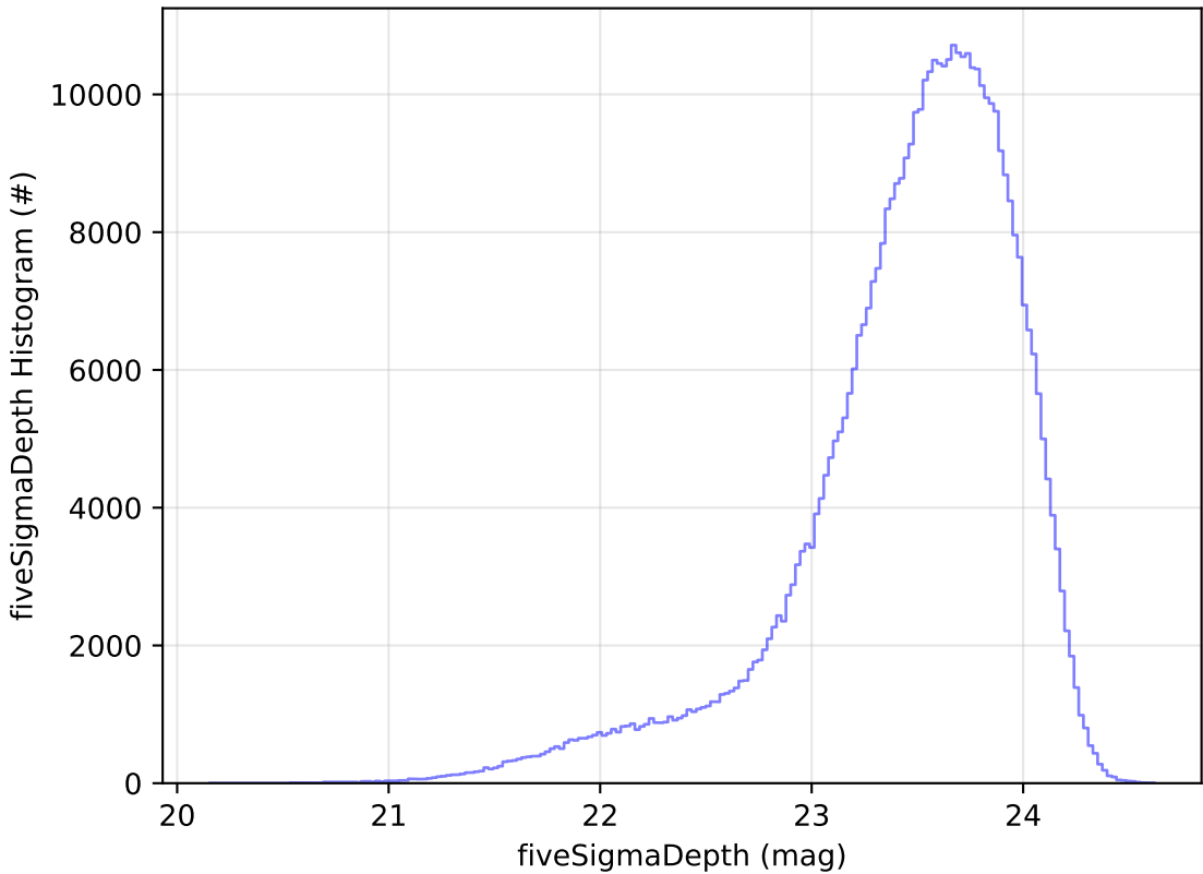
too_elab_r128_d3_gz_v3.4_10yrs i: fiveSigmaDepth Histogram
