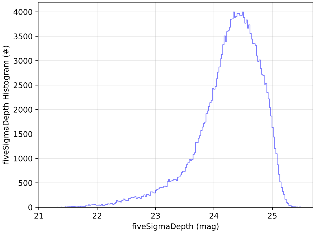
too_elab_r128_d3_gz_v3.4_10yrs g: fiveSigmaDepth Histogram
