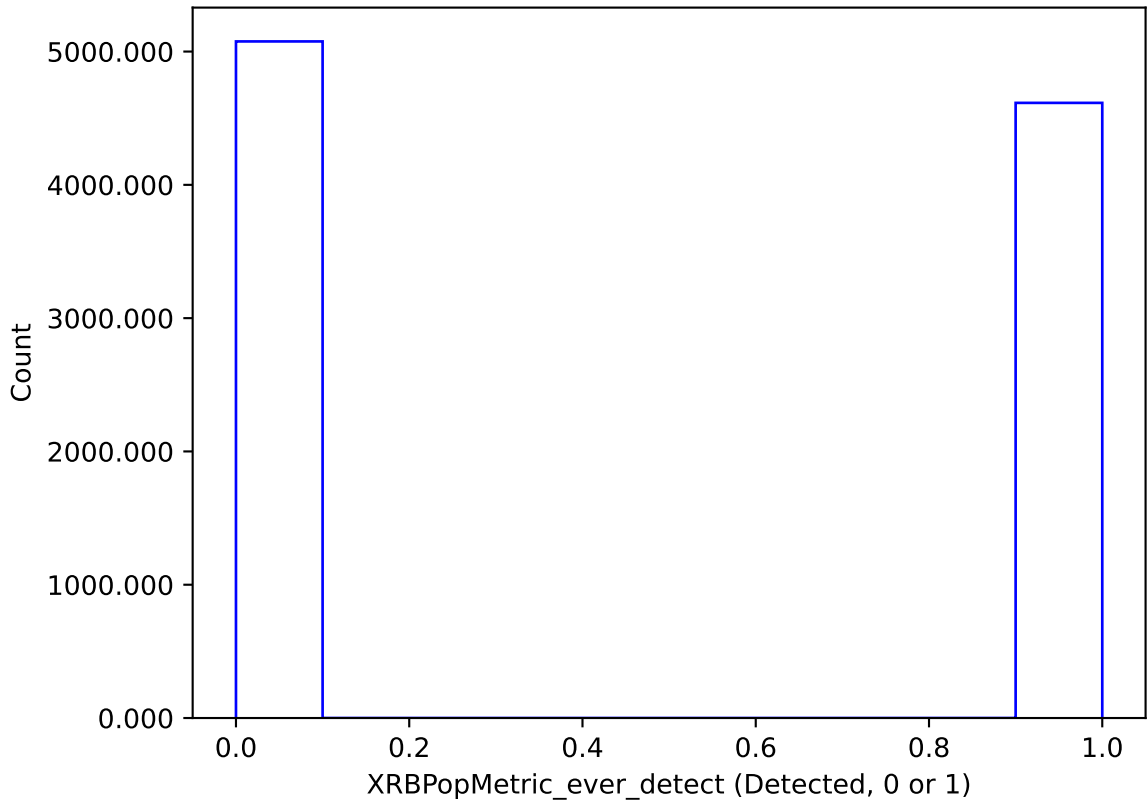
too_elab_r128_d3_gz_v3.4_10yrs : XRBPoMetric_ever_detect
