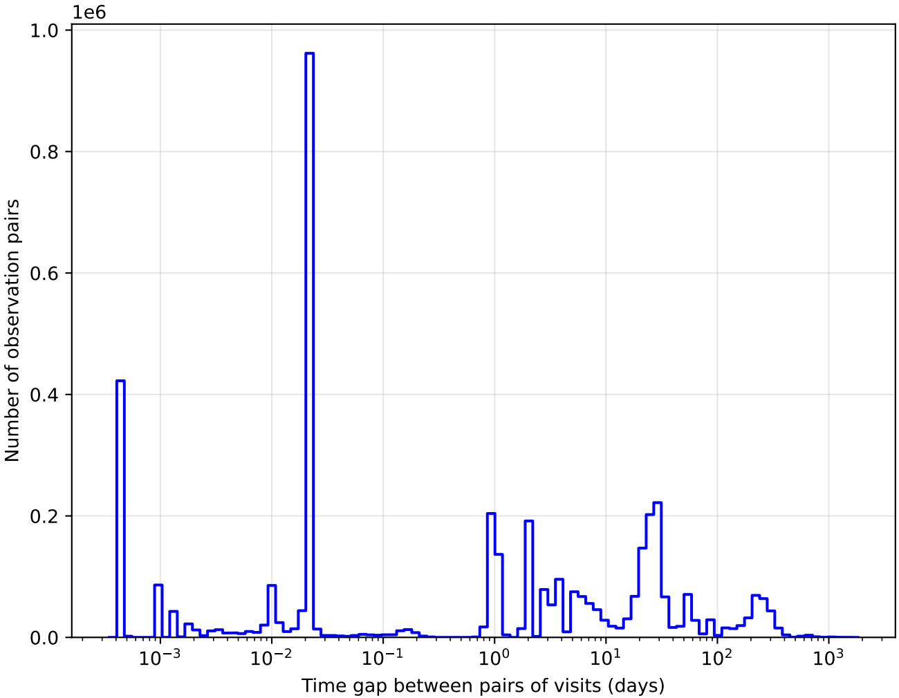
too_elab_r128_d3_gz_v3.4_10yrs y band: Tgaps observationStartMJD
