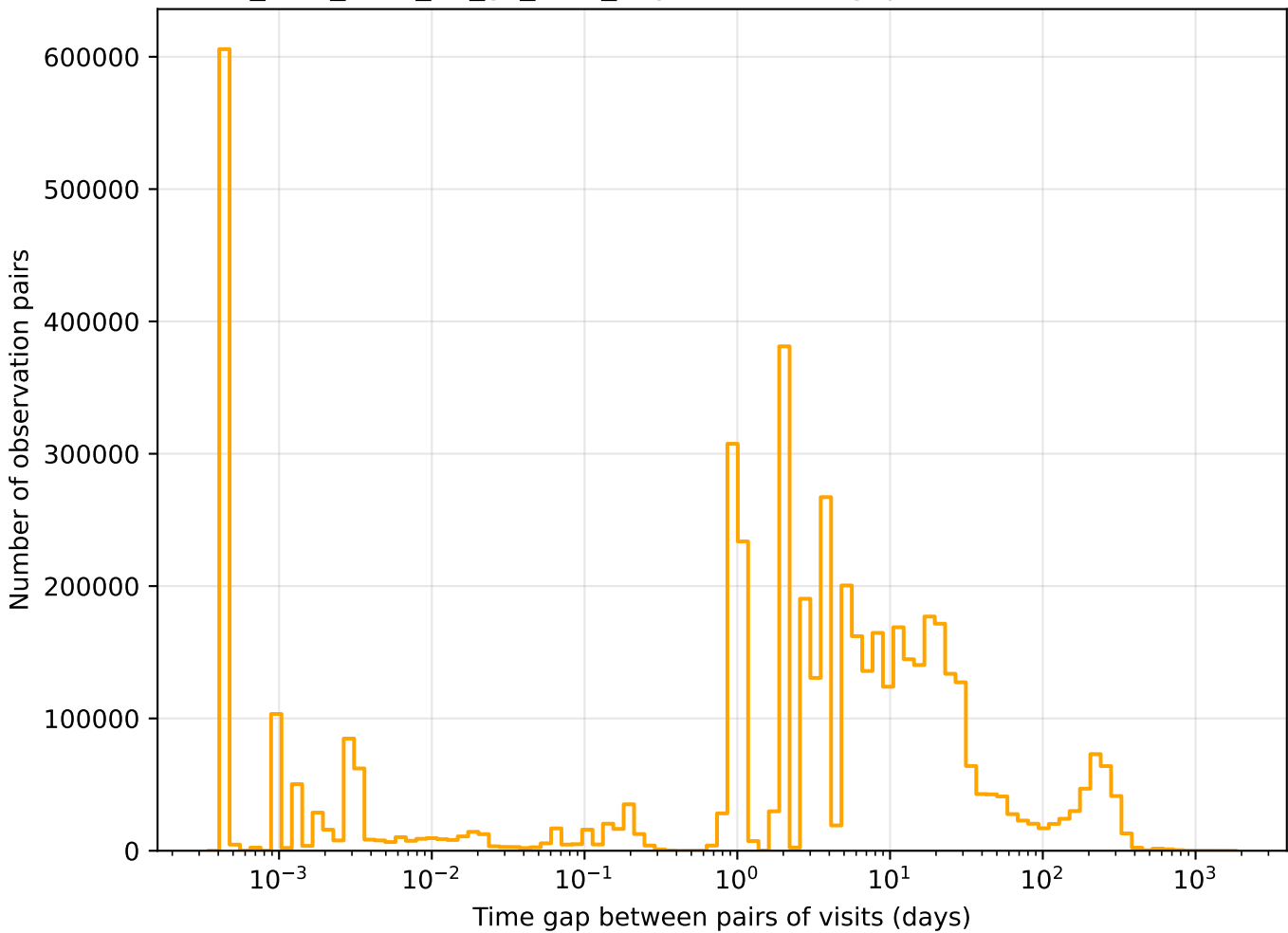
too_elab_r128_d3_gz_v3.4_10yrs r band: Tgaps observationStartMJD
