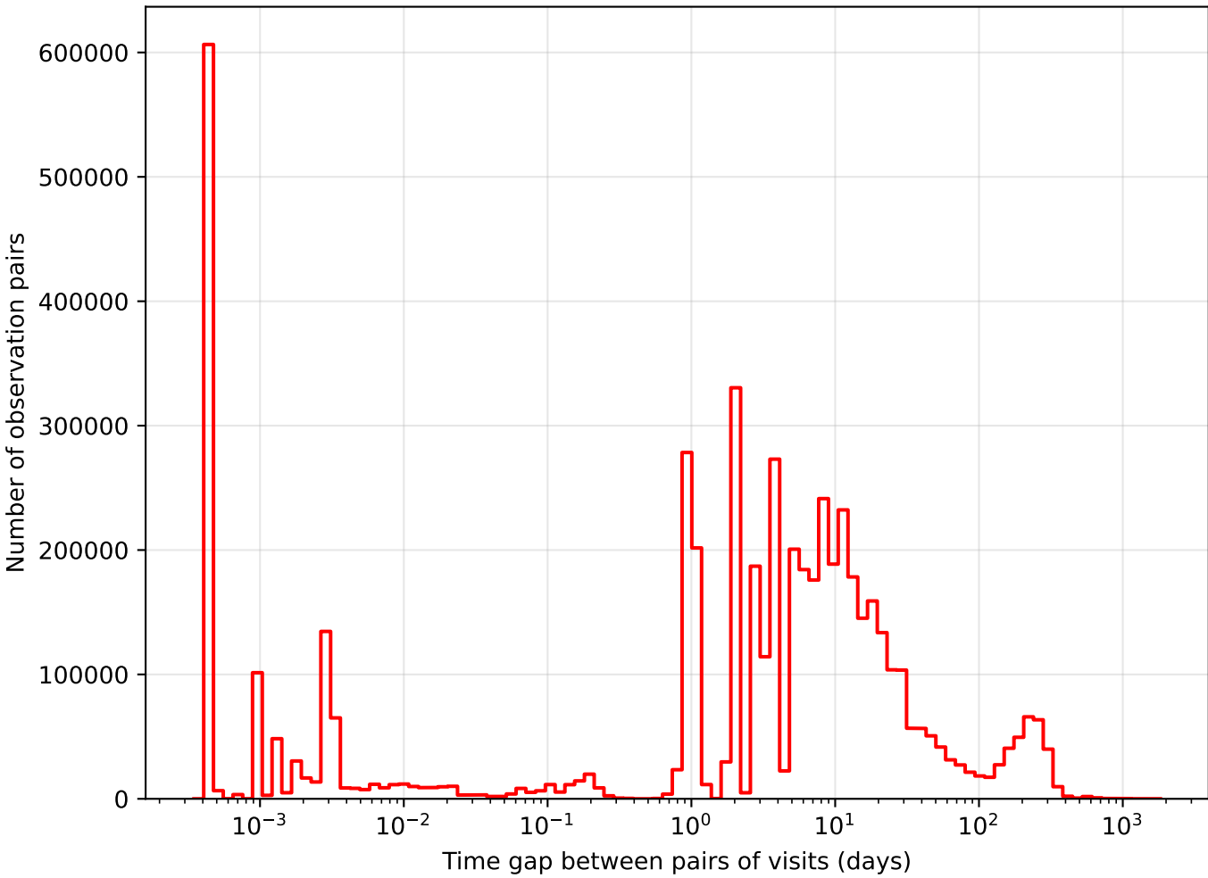
too_elab_r128_d3_gz_v3.4_10yrs i band: Tgaps observationStartMJD
