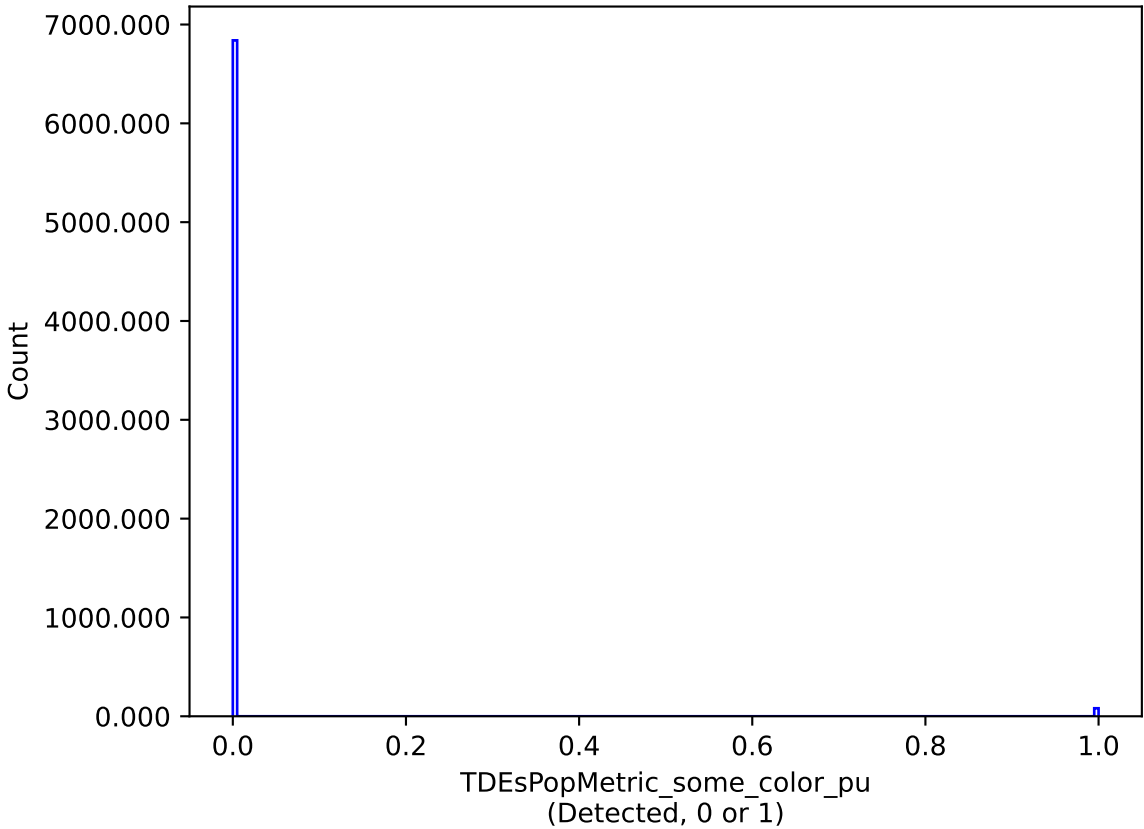
too_elab_r128_d3_gz_v3.4_10yrs : TDEsPopMetric_some_color_pu
