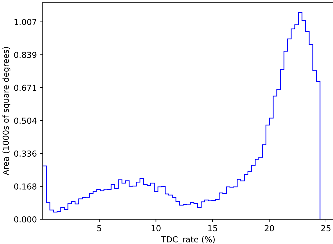
too_elab_r128_d3_gz_v3.4_10yrs : TDC_rate
