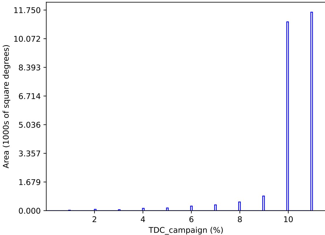
too_elab_r128_d3_gz_v3.4_10yrs : TDC_campaign
