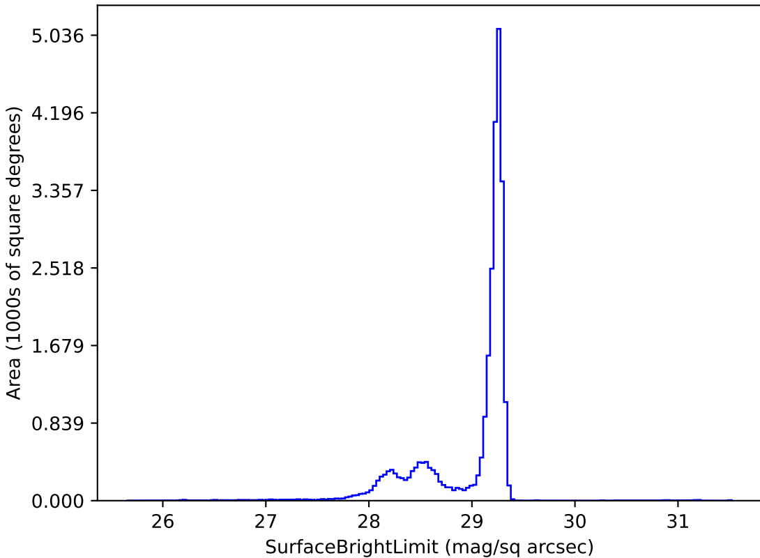
too_elab_r128_d3_gz_v3.4_10yrs z: SurfaceBrightLimit
