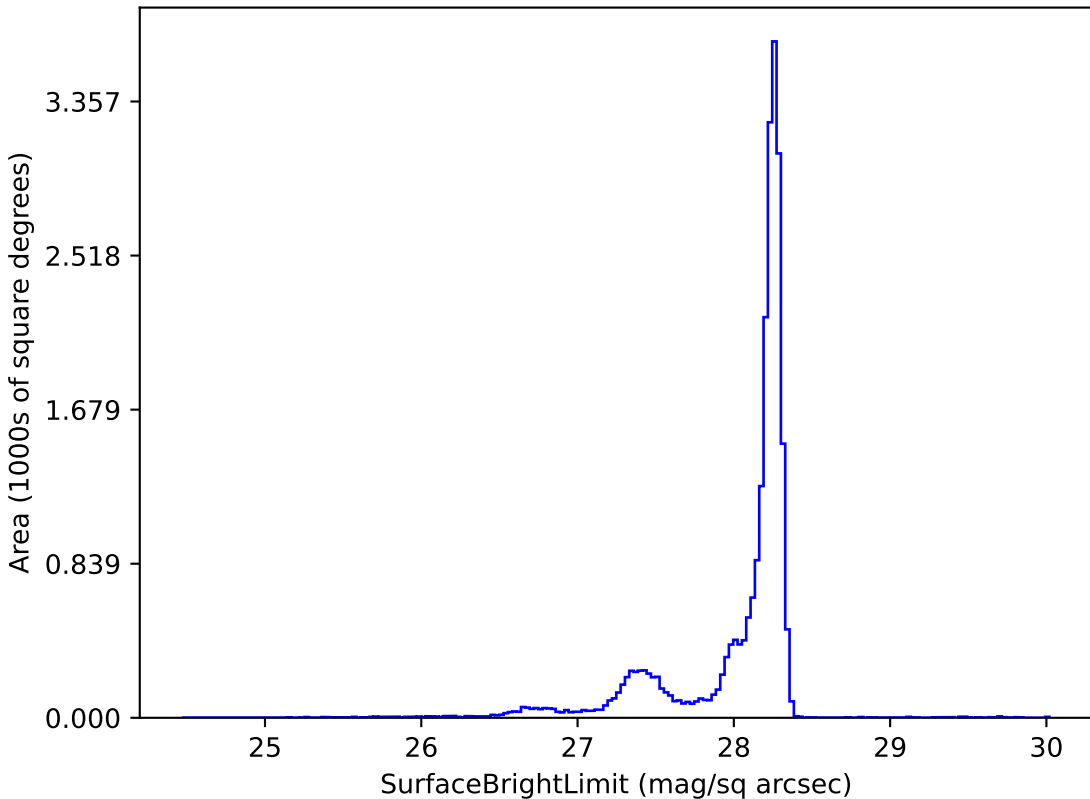
too_elab_r128_d3_gz_v3.4_10yrs y: SurfaceBrightLimit
