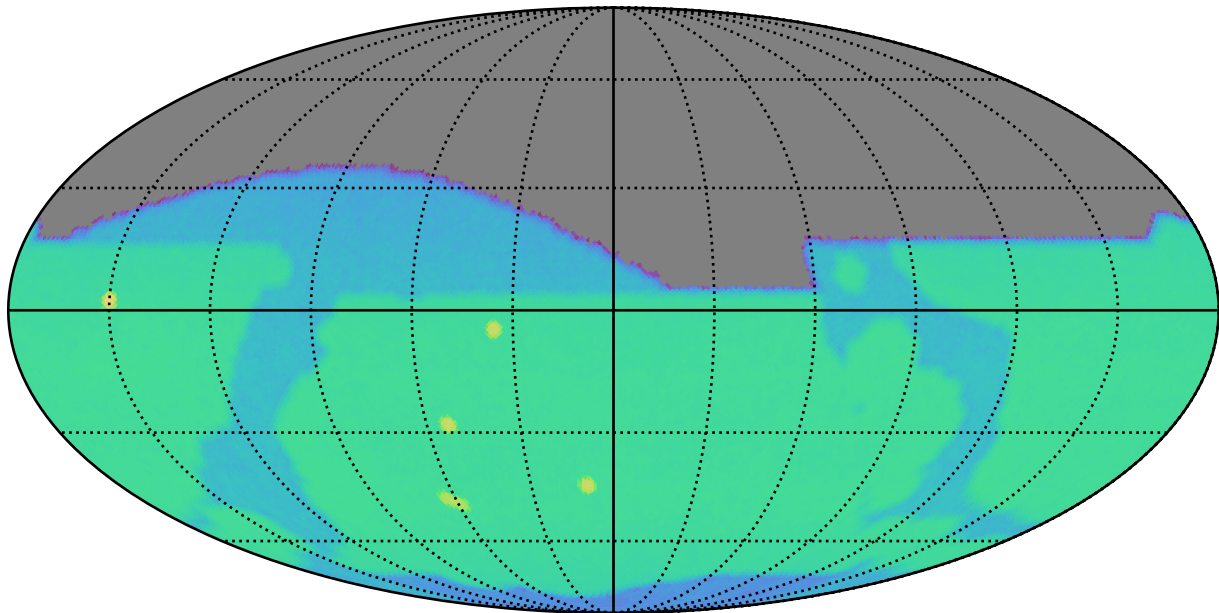
too_elab_r128_d3_gz_v3.4_10yrs i: SurfaceBrightLimit
