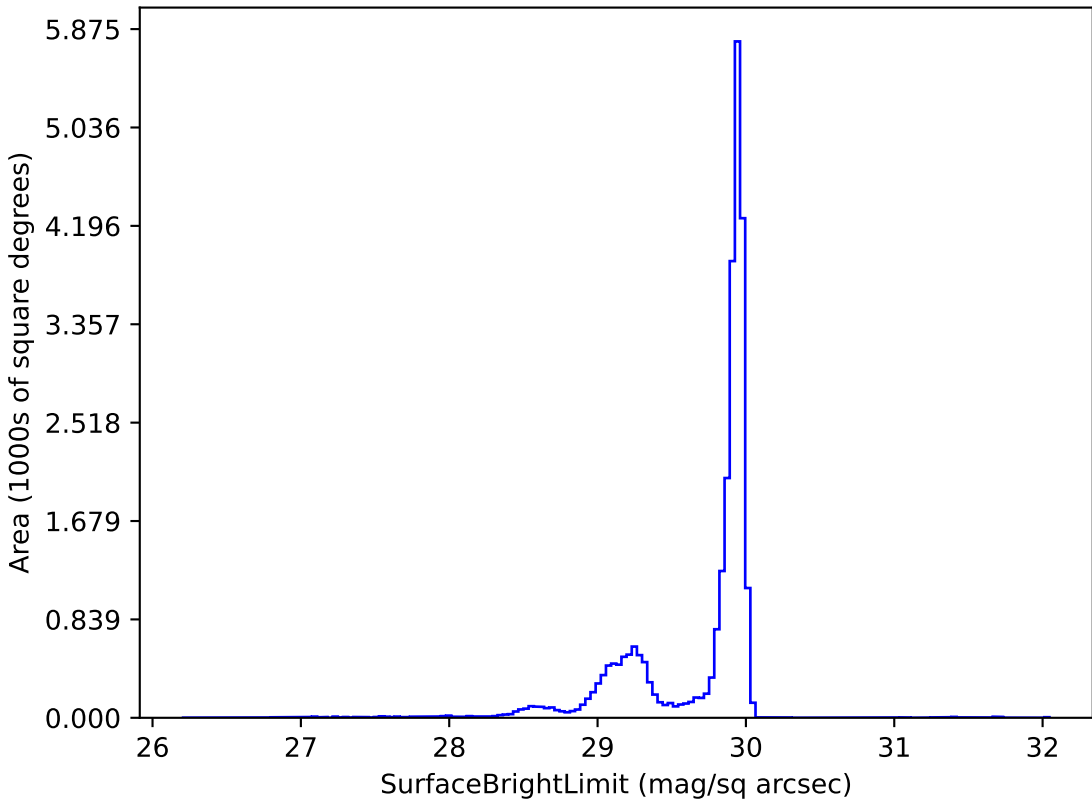
too_elab_r128_d3_gz_v3.4_10yrs i: SurfaceBrightLimit
