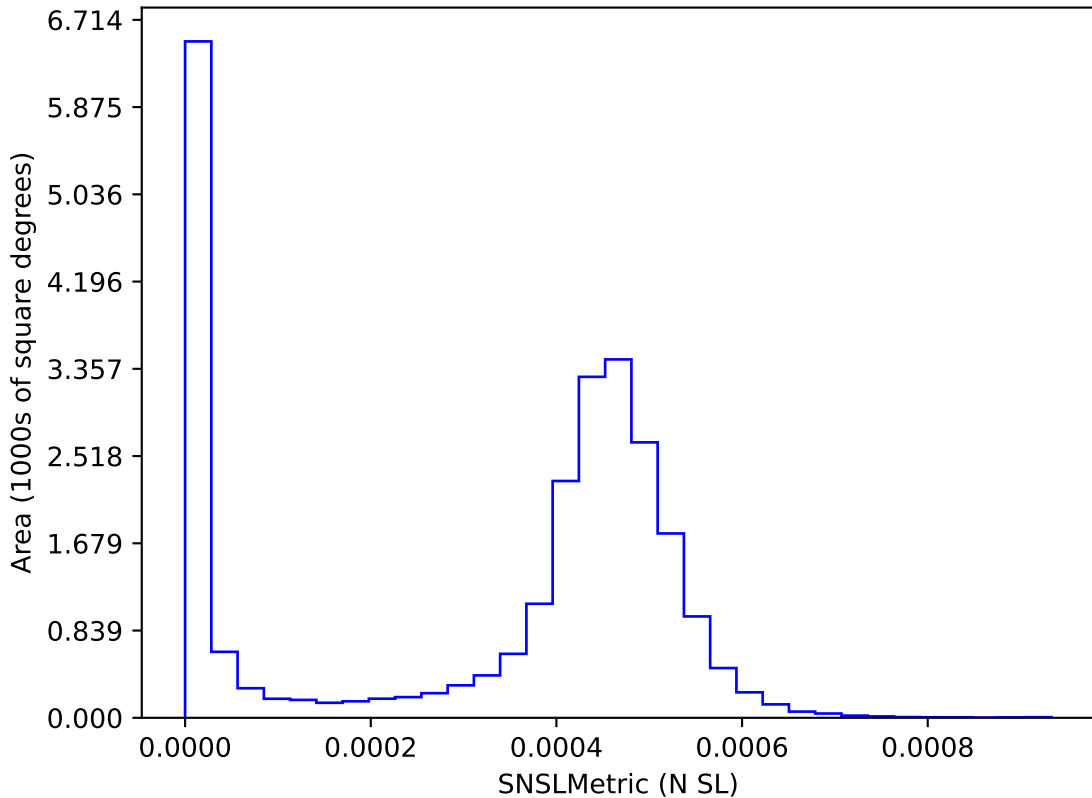
too_elab_r128_d3_gz_v3.4_10yrs : SNSLMetric
