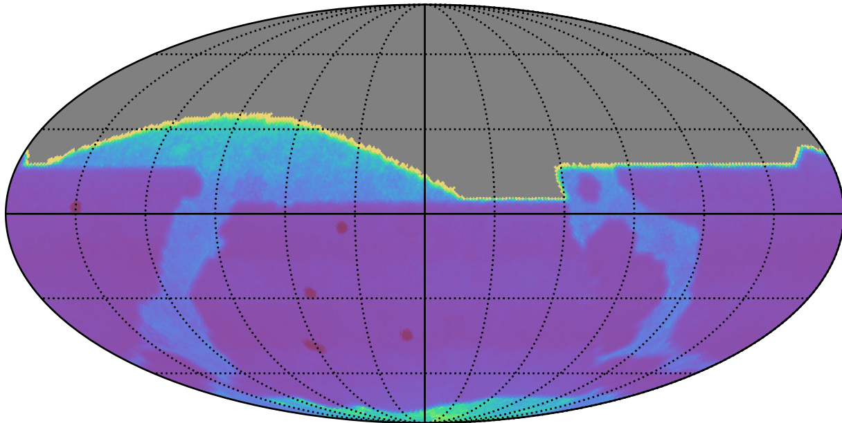
too_elab_r128_d3_gz_v3.4_10yrs : Proper Motion Uncert @ 20.5
