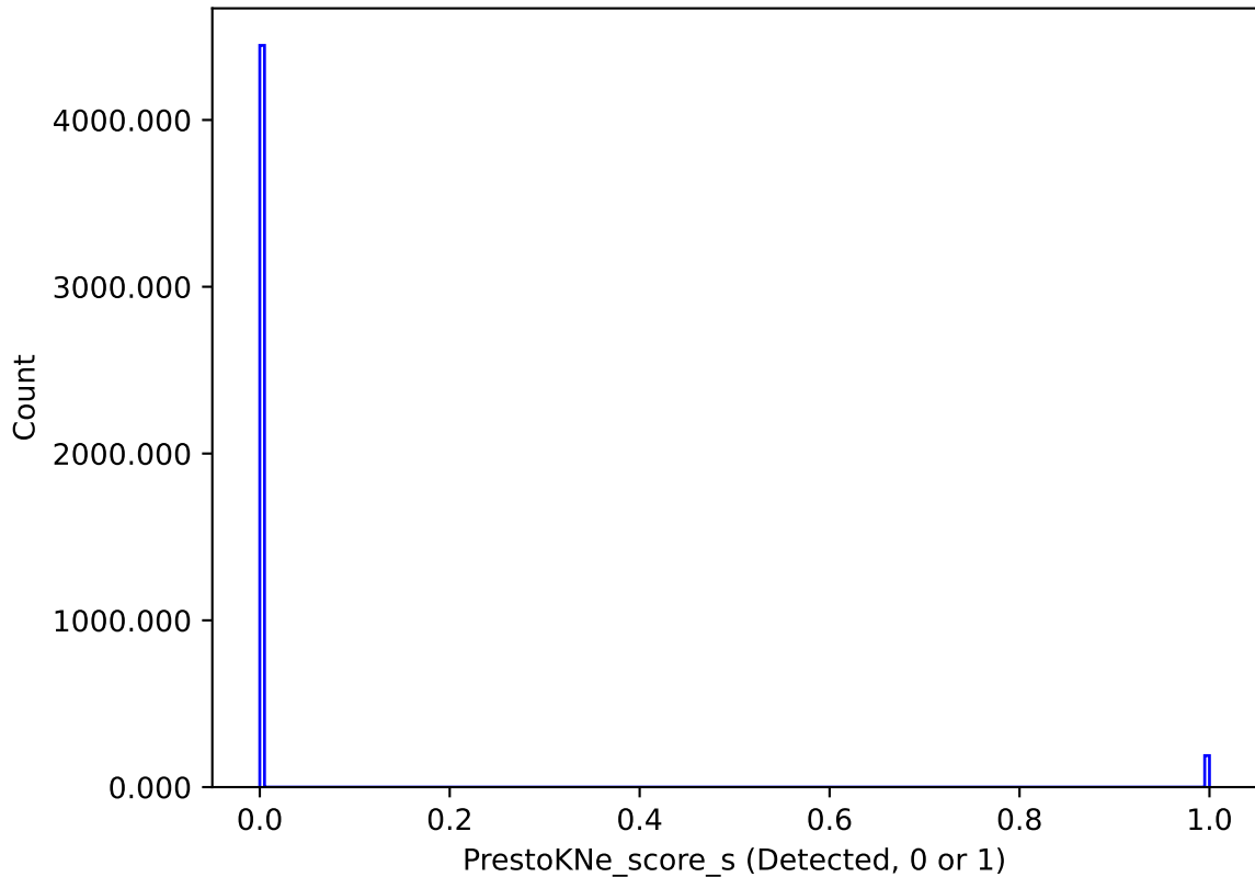
too_elab_r128_d3_gz_v3.4_10yrs : PrestoKNe_score_s
