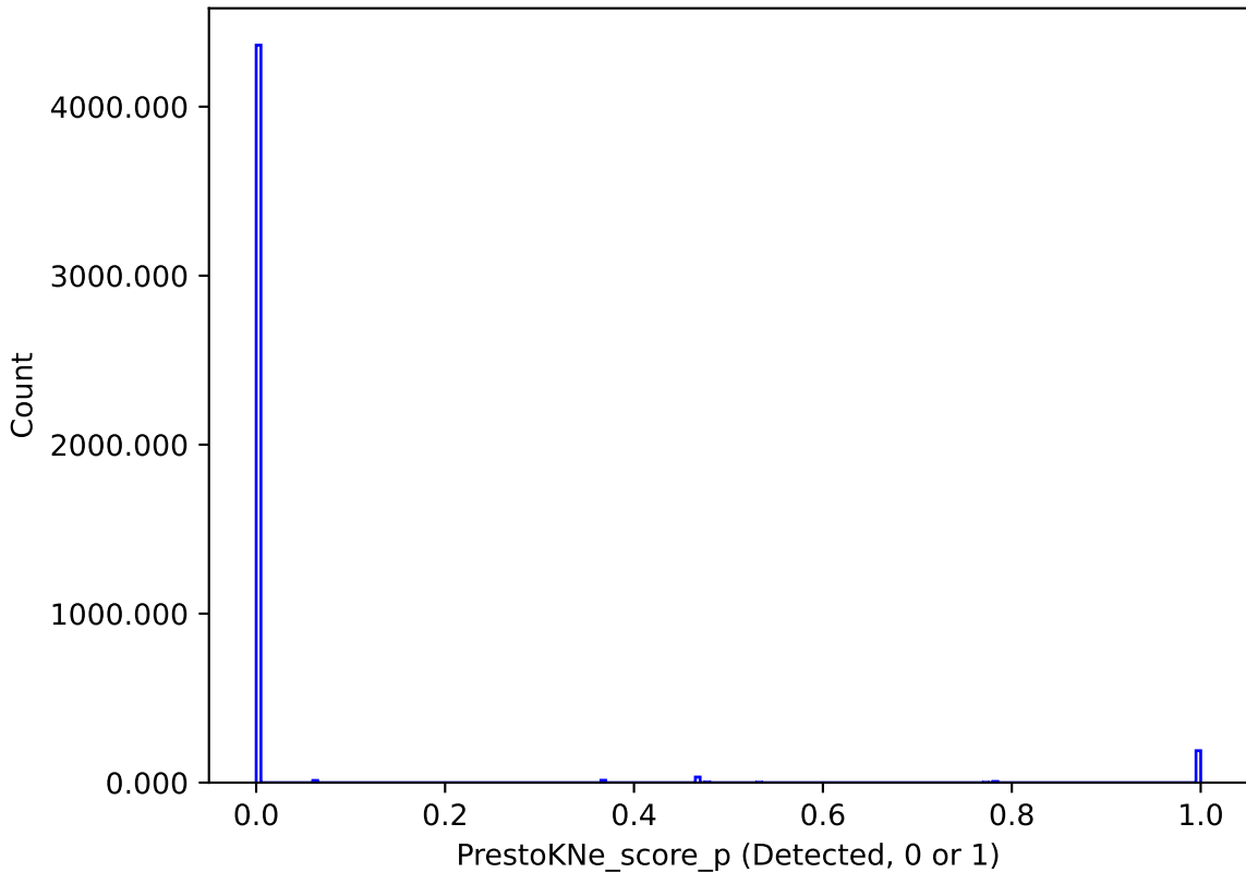
too_elab_r128_d3_gz_v3.4_10yrs : PrestoKNe_score_p
