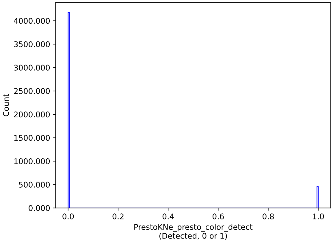
too_elab_r128_d3_gz_v3.4_10yrs : PrestoKNe_presto_color_detect
